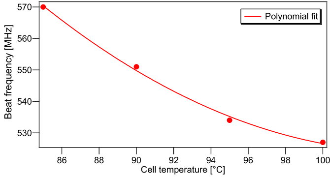
Fig. 7. Beat frequency vs. cell temperature.
