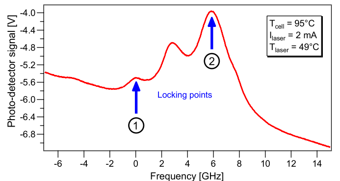
Fig. 5. Doppler-broadened absorption spectrum. The peak labeled 1 corresponds to ^{87}\text{Rb} and the peak labeled 2 corresponds to the ^{85}\text{Rb} .
