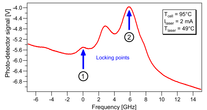
Fig. 5. Doppler-broadened absorption spectrum. The peak labeled 1 corresponds to 87 Rb and the peak labeled 2 corresponds to the 85 Rb.
