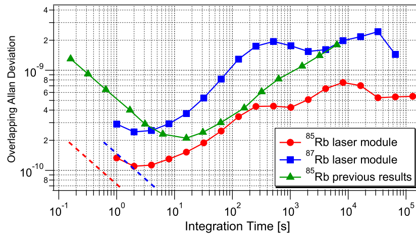
Fig. 9. Frequency stability in terms of Allan deviation for ^{85}\text{Rb} (red dots), ^{87}\text{Rb} (blue squares) and previous results obtained with a bigger setup on ^{85}\text{Rb} (green triangles [16]). The estimated S/N limits are the red and blue dashed lines. (For interpretation of the references to color in this figure legend, the reader is referred to the web version of this article.)
