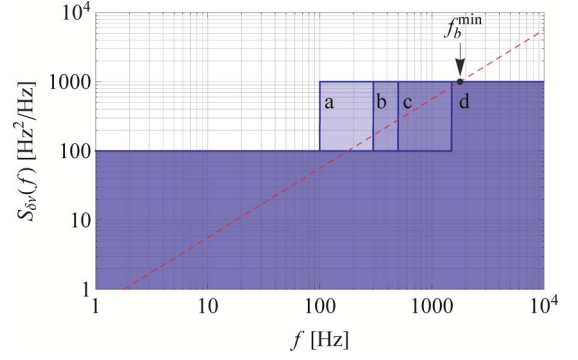
Fig. 6. (Color online) Frequency noise model used to study laser linewidth reduction using a servo loop. We assume that the free-running laser noise level h_b = 1000 \text{Hz}^2/\text{Hz} is reduced to h_a = 100 \text{Hz}^2/\text{Hz} with a servo loop having a bandwidth f_b of a, 100 Hz; b, 300 Hz; c, 500 Hz; and d, 1500 Hz. The dashed line represents the \beta -separation line. The minimum servo-loop bandwidth necessary to efficiently reduce the laser linewidth is f_b^{\min} = \pi^2 h_b / (8 \ln(2)) .
