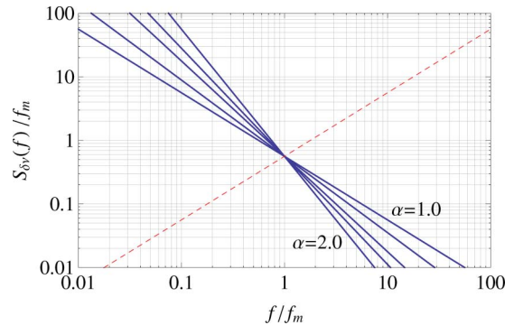
Fig. 4. (Color online) Pure flicker frequency noise model of Eq. (11) with \alpha = 1, 1.2, 1.5, 1.7, \text{ and } 2.0 . The axes are normalized with respect to the frequency f_m , at which S_{\delta\nu} intersects the \beta -separation line.
