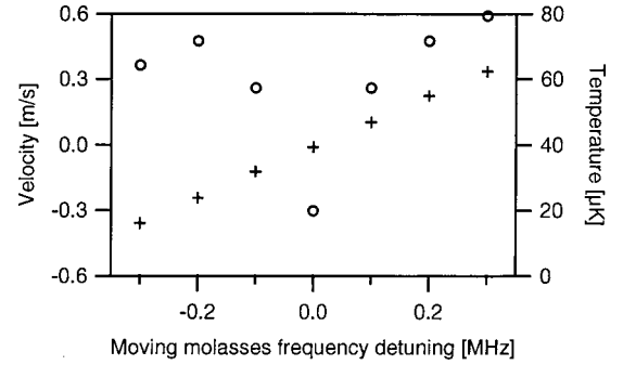
FIG. 8. Mean velocity \bar{v}_z (+) and longitudinal temperature T (O) in the cold atom source as a function of moving molasses detuning \Delta/2\pi . These values of \bar{v}_z and T have been computed from the center and distance between peaks of the RIR.
