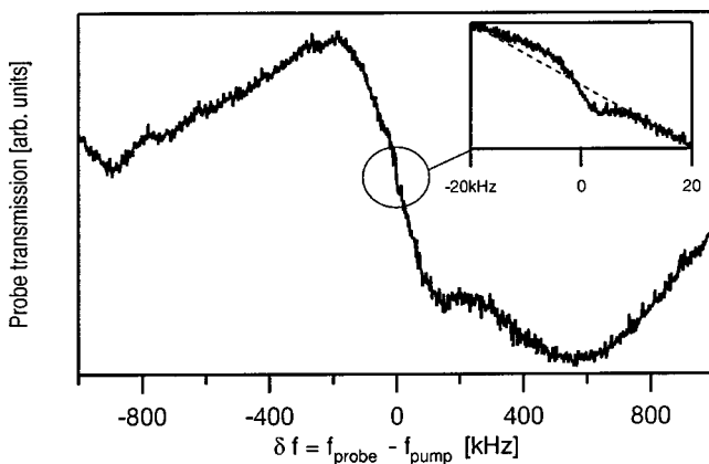
FIG. 7. Probe transmission spectrum in the 2D MOT source for zero-moving molasses frequency detuning. It is still possible to distinguish a small recoil-induced resonance in the spectrum center as shown in the inset.
