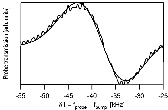
FIG. 4. Probe transmission spectrum in an atomic beam launched at 1.205 m/s (1 MHz detuning). We observe a recoil-induced resonance centered at -38 kHz whose distance between peaks is approximately 10 kHz. The smooth line is a Gaussian derivative fit corresponding to a velocity \bar{v}_z = 1.3 m/s and longitudinal temperature T = 510 \mu\text{K} .
