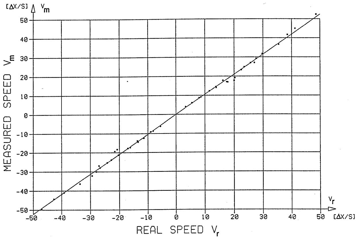
FIGURE 9: OPTICAL FLOW LINEARITY
