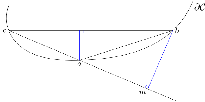
FIG. 10 – Cas a \in [m, c]
